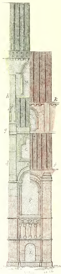
Fig. 16. Exterior Elevation.
